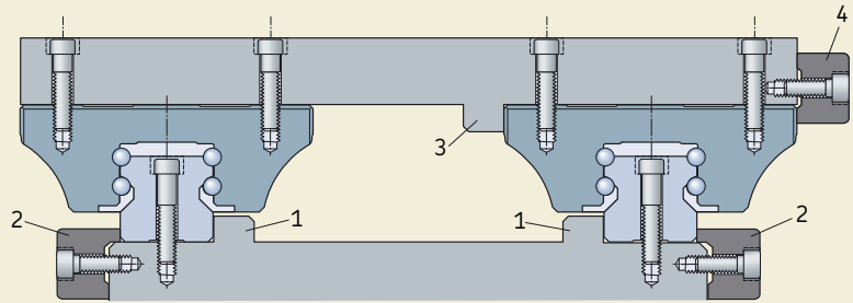
Mounting with laterally fixed rails and carriages
