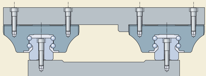
Mounting without lateral rail fixation
