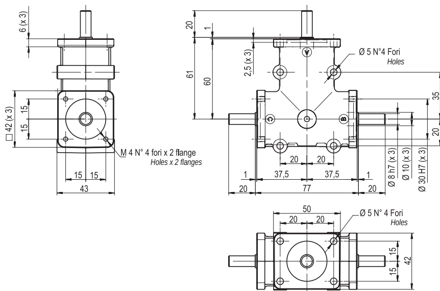
MISURA 2 SIZE 2 MOD. RP
