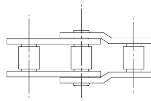
Double offset link
