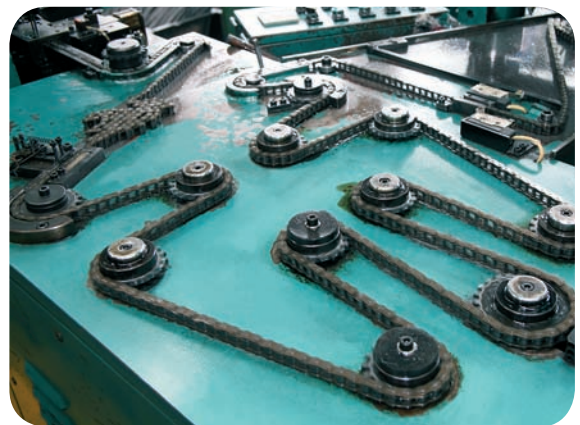
Automated chain assembly to ensure proper fits and tolerances are met.
