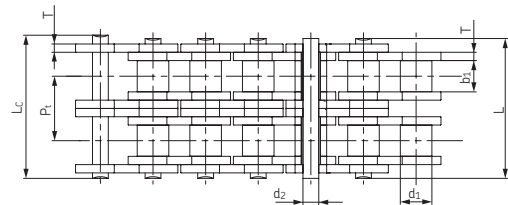
SKF Xtra Strength SH Chains used in the earthmoving industry
