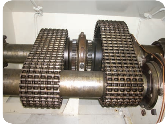
Multiple strands of oil field chain inside a mud pump
