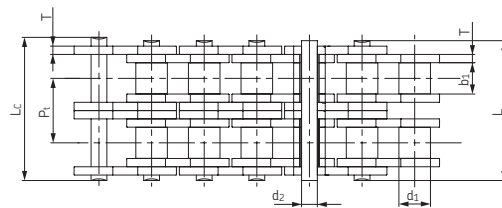
SKF Xtra Strength SHH Chains used in construction machinery
